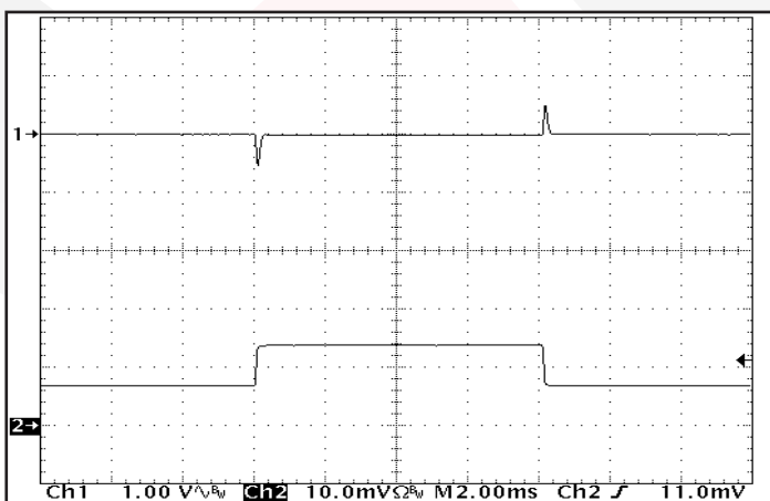
Figure 11: Output voltage response to step-change in load current 50%-100%-50% of Iout (max). Load cap: 1 \mu F ceramic cap and 10 \mu F, 100m \Omega ESR tantalum cap. Ch 1: Vout (1V/div). Ch 2: Iout (10A/div).
